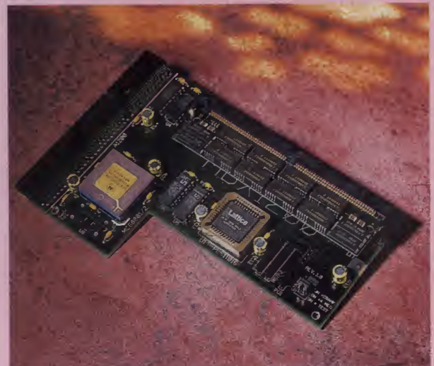
The MicroBotics MBX1200, showing off its 68881 co-processor, and the 4Mb SIMM fitted to the review model.
